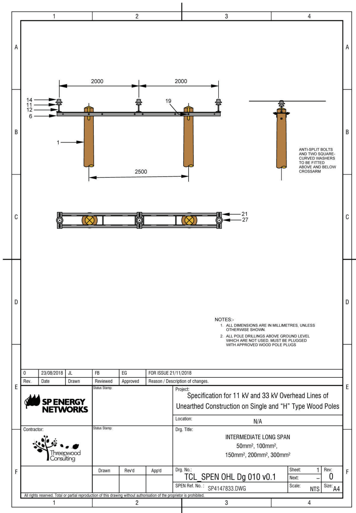
22.10 Figure 10 General Arrangement “H” Pole Intermediate Long Span (Drawing No. SP4147833)
